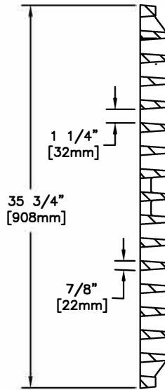
GRATE SECTION
