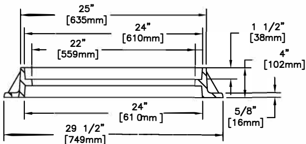
FRAME SECTION
