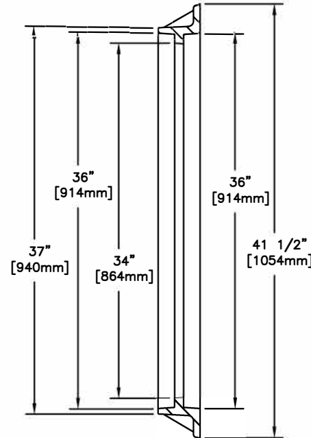
FRAME SECTION
