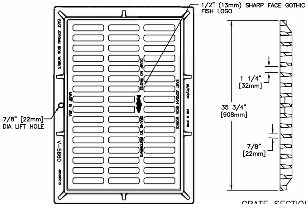
GRATE SECTION
